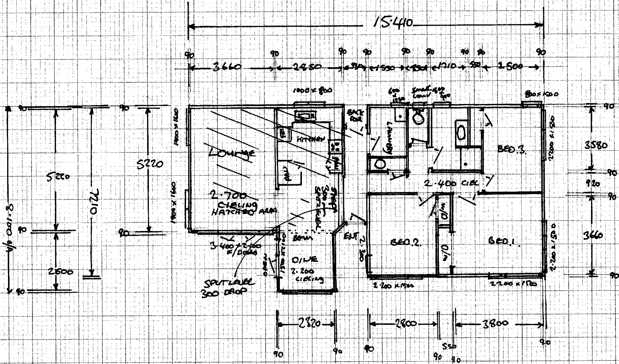
FLOOR PLAN (TONI) TIRI MOANA RD.
