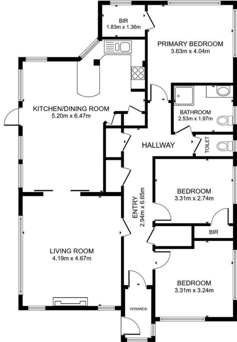
FLOOR PLAN
